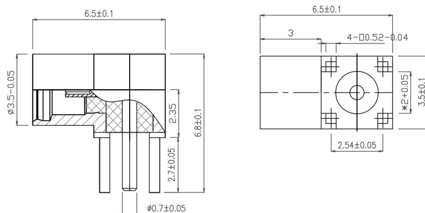
Figure 1: MM0N9T0G-CA
