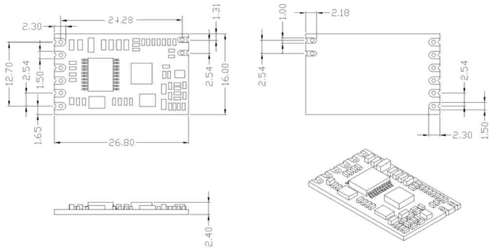
Figure 6: DRF4432D20I-M2 Dimension
