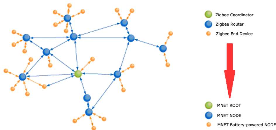
Figure 31: Replace Zigbee with MNET III Network
