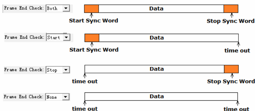
Figure 17: Synchronization Words in ASCII Frame Mode.
