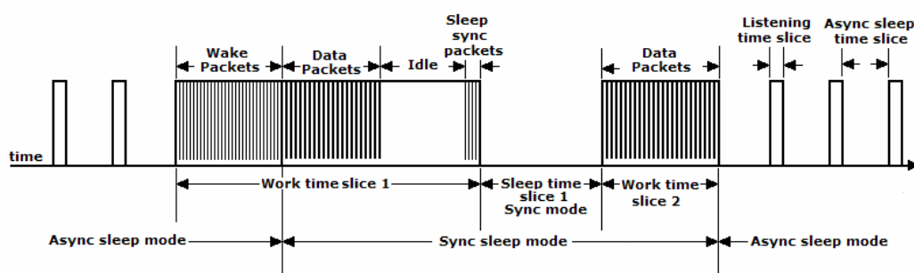
Figure 25: Wake-up Packets in Hybrid Sleep Mode
