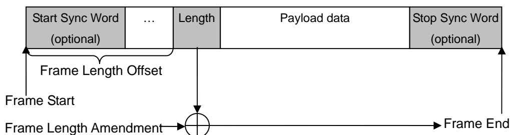
Figure 19: Variable Frame Length in Binary Mode
