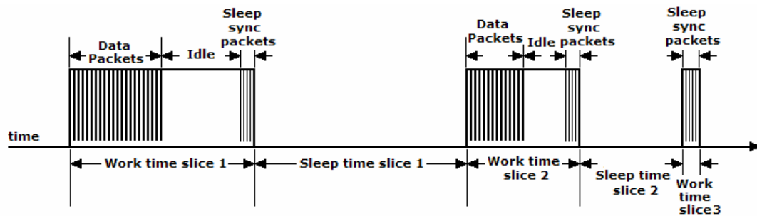
Figure 15: Synchronous Sleep Interval
