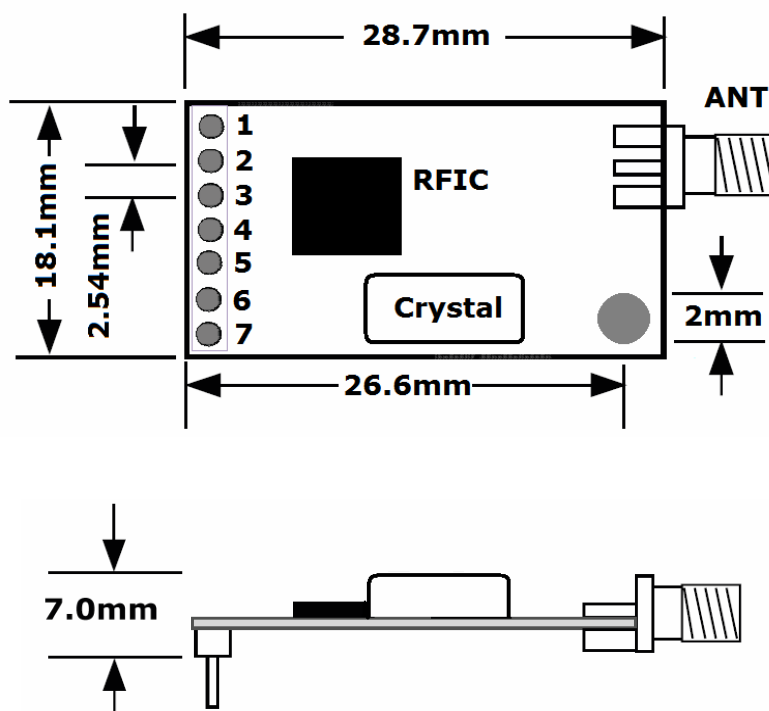
Figure 34: Mechanical Dimensions
