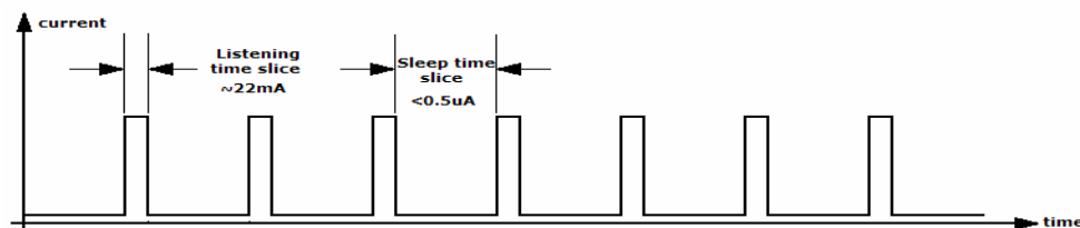
Figure 22: Power Consumption in Asynchronous Sleep Mode
