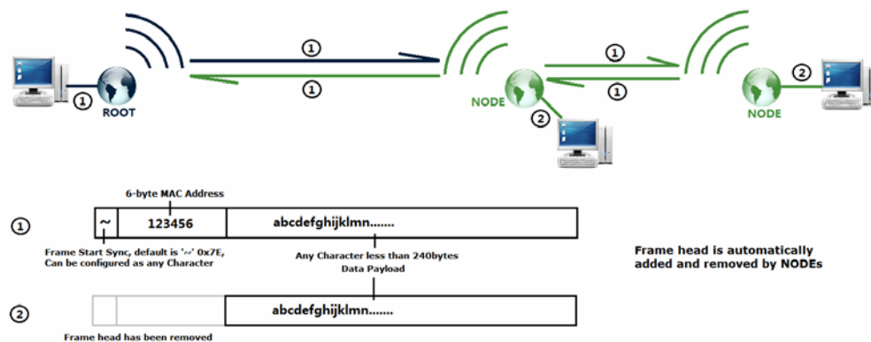
Figure 12: Frame Structure of Half Transparent Transmission
