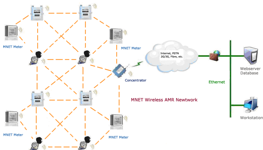
Figure 28: Wireless AMR Network Based on MNET III
