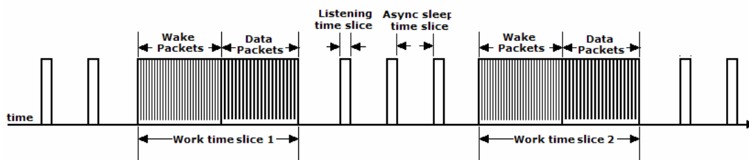
Figure 23: Wake-up Packets in Asynchronous Sleep Mode
