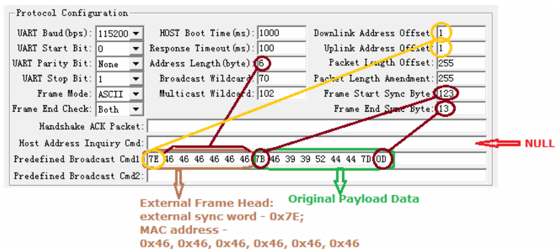
Figure 21: Predefined Broadcast CMD1 & MAC Address
