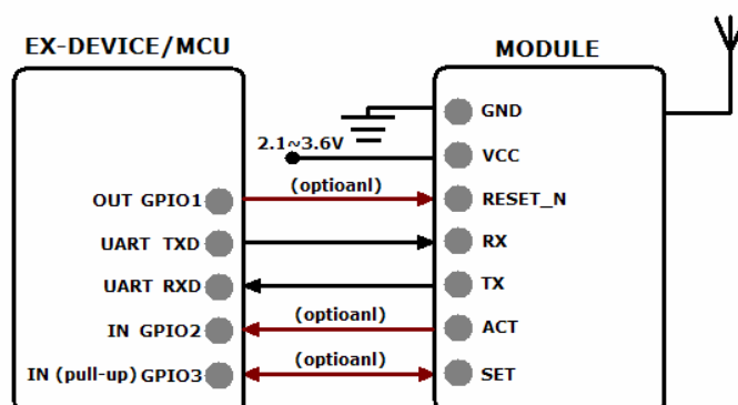
Figure 8: DRF1110N Connection Diagram
