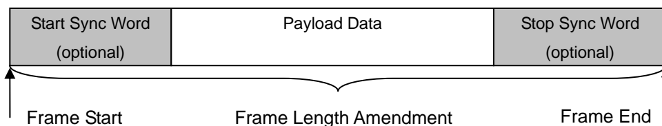
Figure 18: Fixed Frame Length in Binary Mode
