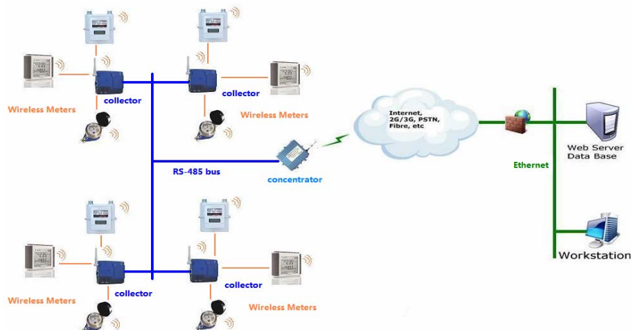
Figure 27: Typical Wireless AMR Network
