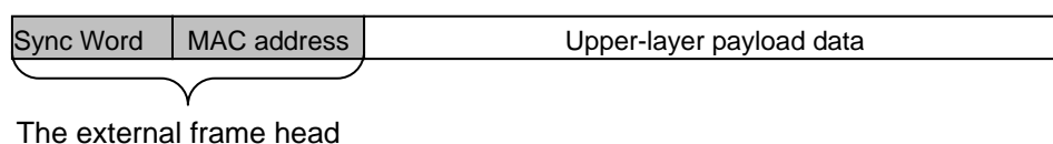
Figure 20: External Frame Head Structure
