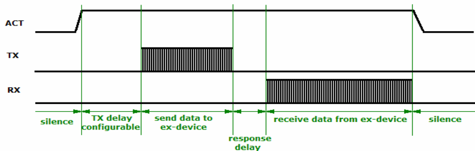
Figure 16: Time Sequence for TX Delay
