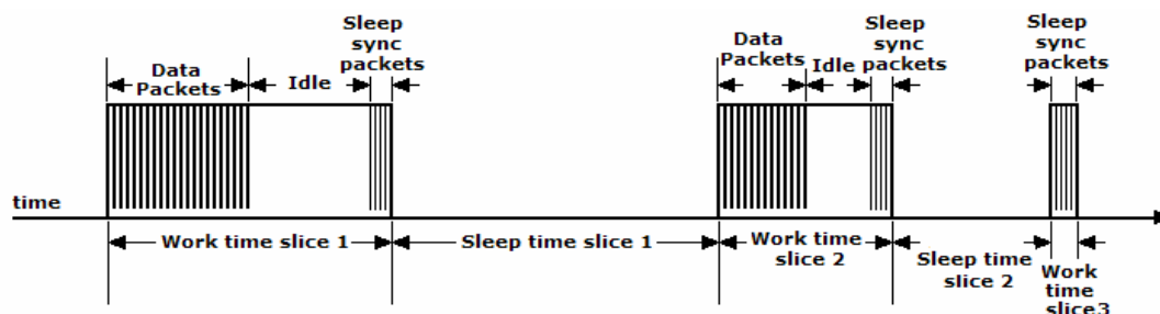
Figure 24: Wake-up Packets in Synchronous Sleep Mode
