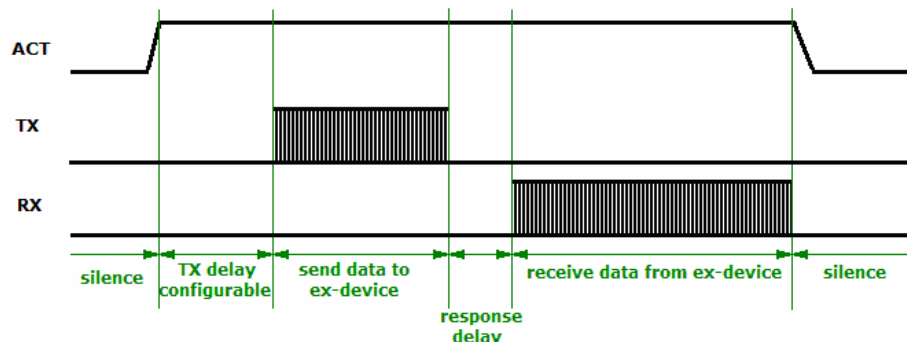
Figure 10: Two-way Communication of ACT, TX and RX Pins
