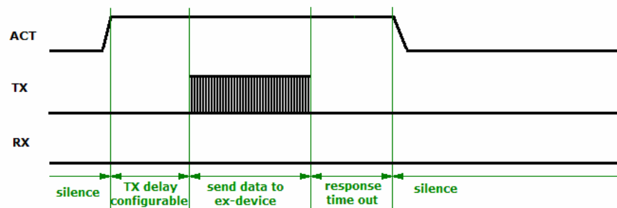
Figure 11: One-way Communication of ACT, TX and RX Pins
