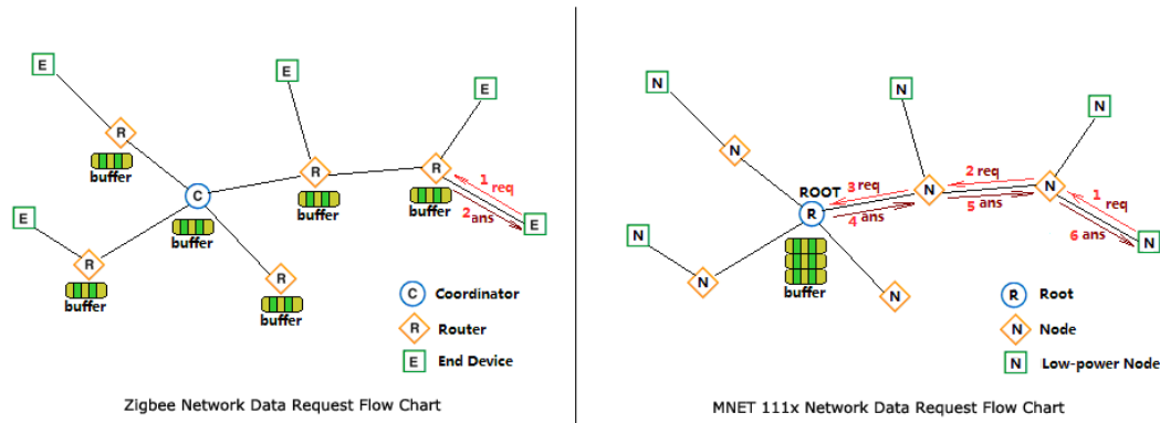
Figure 32: Zigbee Vs MNET III in Data Flow
